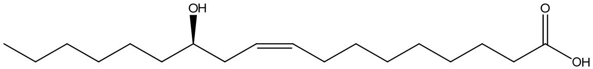
Figure 25: Ricinoleic Acid Molecule
