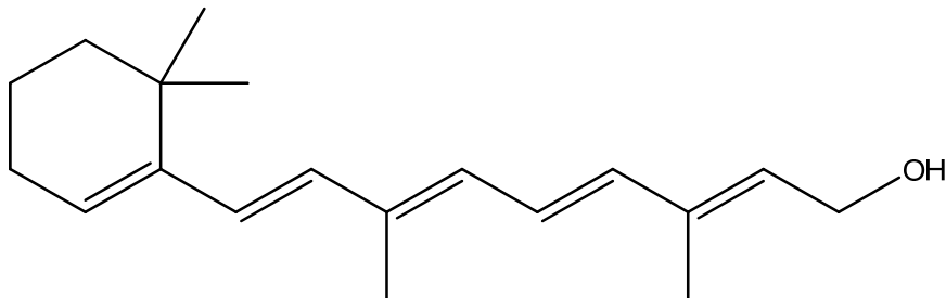
Figure 23: Retinol Molecule
