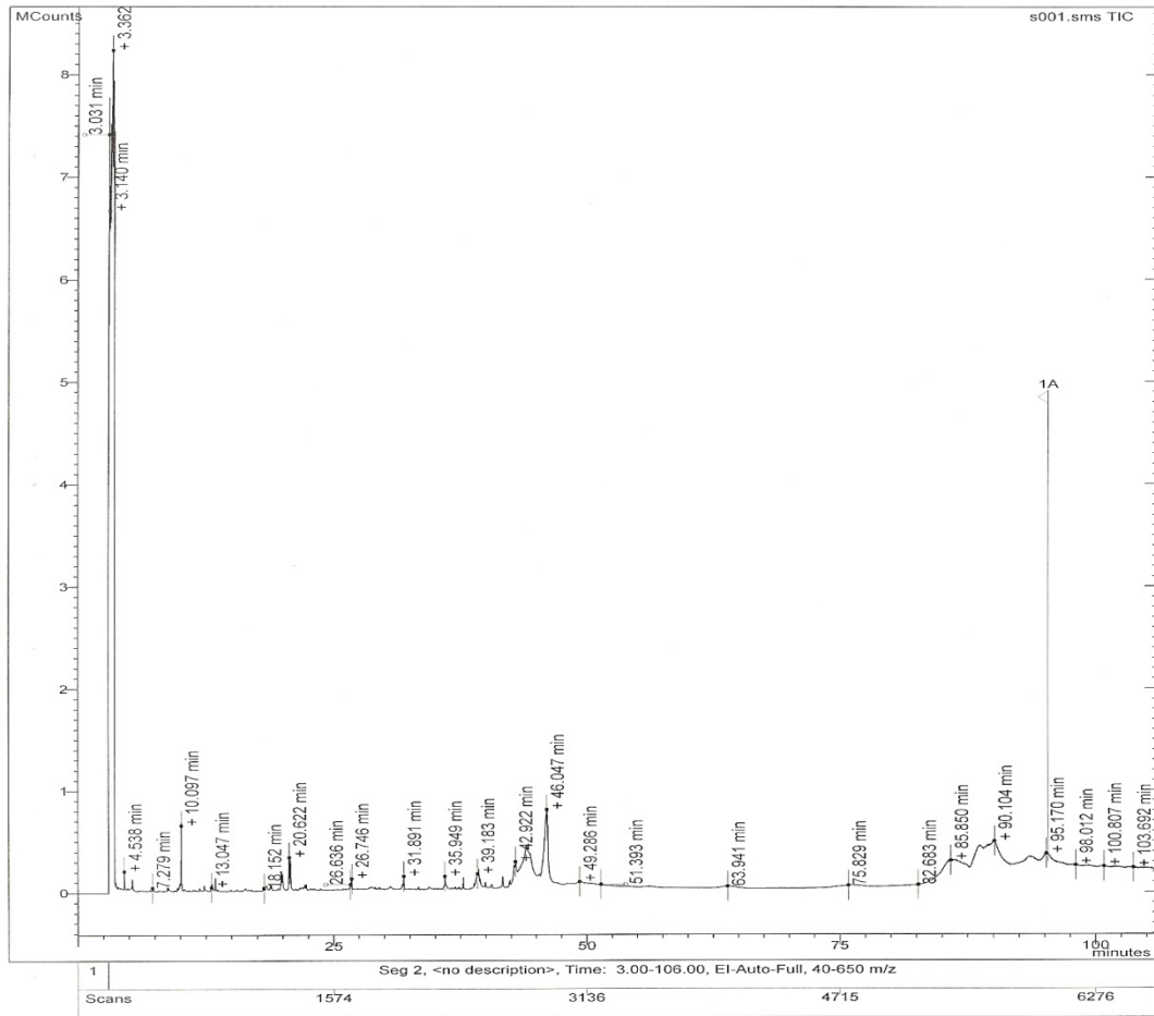
Figure 12: GC of BB Sample at 125 Bars and 46.9°C
