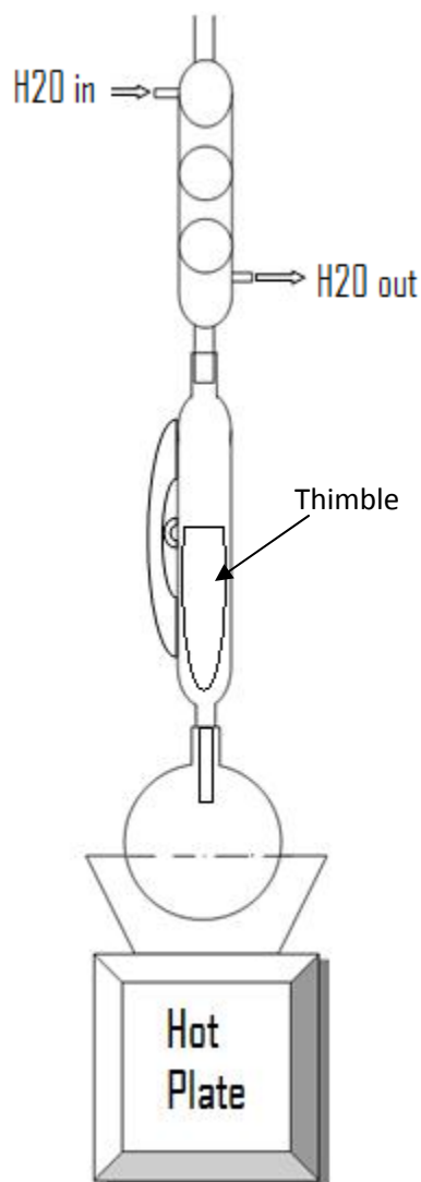
Figure 7: Soxhlet Extraction Setup
