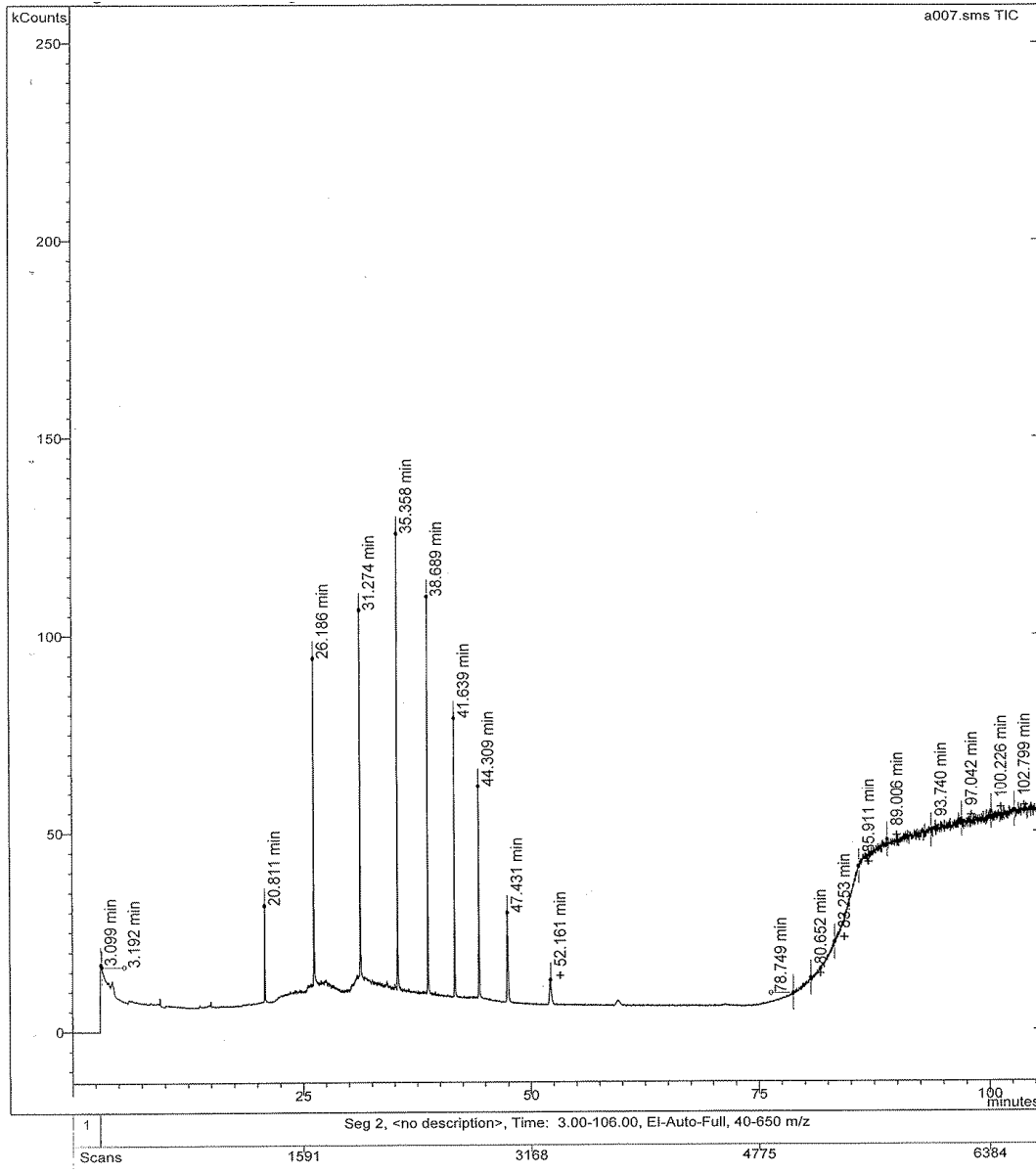
Figure 18: GC of CB Sample at 194 Bars and 50.4°C
